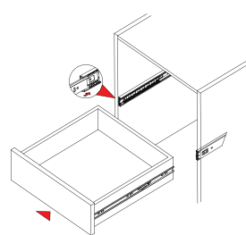
Plastic rear socket: JZZH01
